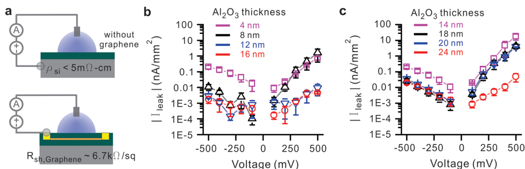
Figure 2. Leakage test on various thicknesses of \text{Al}_2\text{O}_3 . (a-top) Schematics showing leakage measurement setup for \text{Al}_2\text{O}_3 on p++ silicon ( \rho < 5 \text{ m}\Omega\text{-cm} ). \text{Al}_2\text{O}_3 of thickness 4 to 16 nm was deposited on the conductive Si wafer. Measurements are conducted with one electrode connected to Si wafer and the other attached to Ag/AgCl electrode in the solution (a-bottom). Schematic of leakage measurement setup for \text{Al}_2\text{O}_3 on graphene transferred onto Si surface with \text{Al}_2\text{O}_3 deposited on top. \text{Al}_2\text{O}_3 thickness in the range of 14–24 nm is deposited on graphene ( R_{\text{sh}} \approx 6.7 \text{ k}\Omega/\text{sq} ) transferred on a Si wafer with an ALD-deposited \text{Al}_2\text{O}_3 top surface. Measurements are conducted between the graphene film contacted with aluminum wires and the solution contacted with Ag/AgCl electrodes. All leakage experiments are performed in 1 M KCl, 10 mM Tris, 1 mM EDTA at pH 7.6, and at room temperature ( 22 \pm 2 \text{ }^\circ\text{C} ). (b) Leakage current density measured for \text{Al}_2\text{O}_3 on conductive silicon. \text{Al}_2\text{O}_3 thickness less than 10 nm showed leakage current greater than 1 \text{ nA}/\text{mm}^2 at 500 mV, but thicker \text{Al}_2\text{O}_3 ( >10 \text{ nm} ) showed much greater insulation over the voltage range of -500 to +500 \text{ mV} . (c) Leakage current density for \text{Al}_2\text{O}_3 deposited on graphene. Leakage current is observed to be fairly high up to 20 nm-thick \text{Al}_2\text{O}_3 . Also the leakage is significantly higher for positive voltage at Ag/AgCl electrode. \text{Al}_2\text{O}_3 at 24 nm thickness displays decent insulation from leakage. Current leakage occurrence at relative thicker \text{Al}_2\text{O}_3 deposited on graphene is associated with wrinkles on graphene (Supporting Information, Figure S9).
